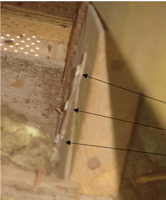
Single strap with at least 3 nails into the truss
